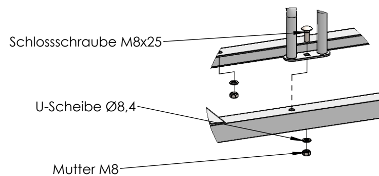
DETAIL A
