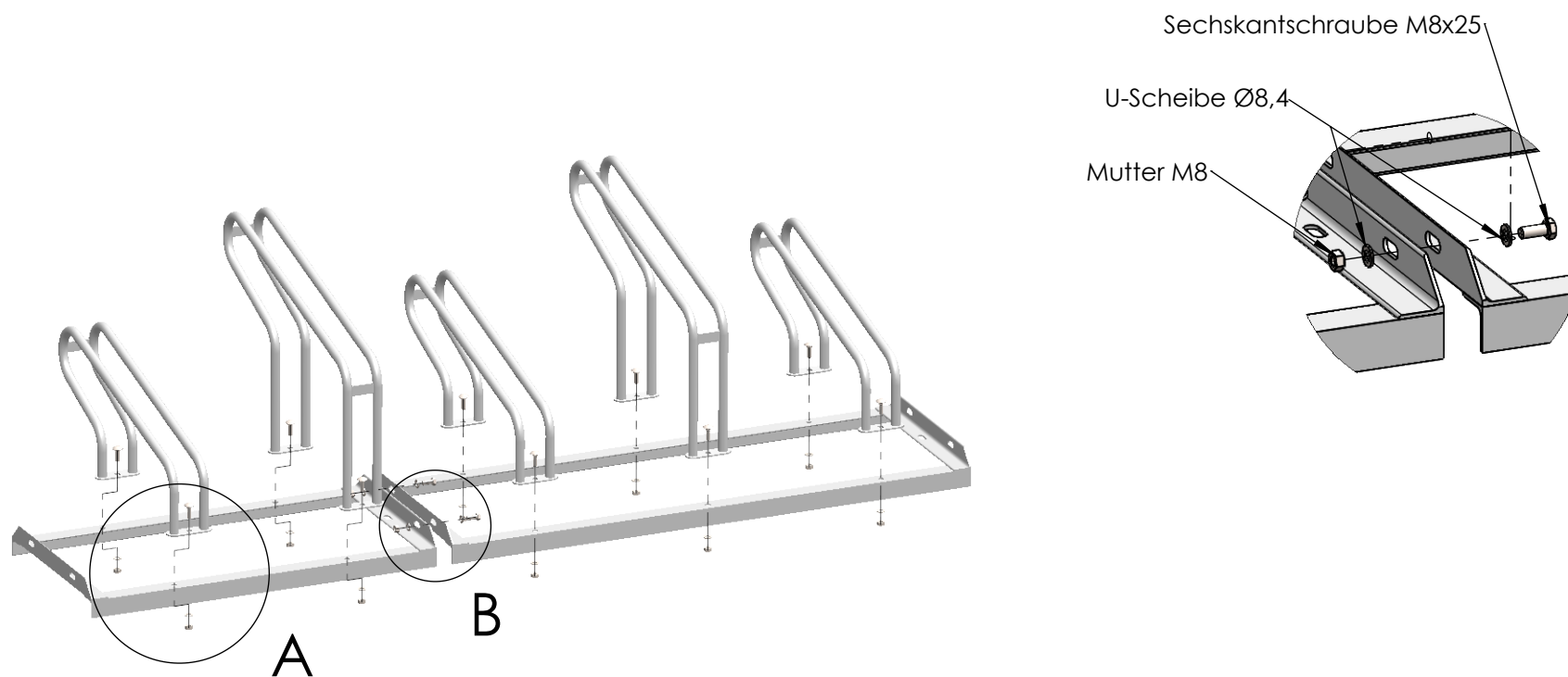
DETAIL B
